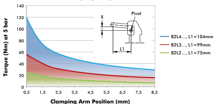
Maximum Clamping Torque at 5 bar
