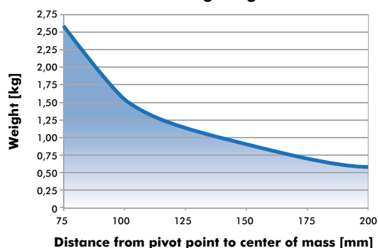
Maximum Tooling Weight 82L4.-2...
