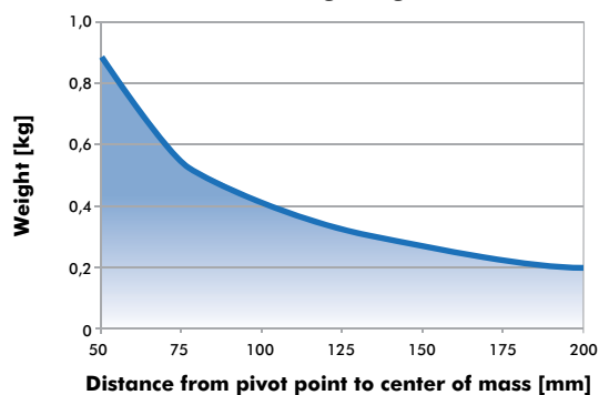
Maximum Tooling Weight 82L2G-2...
