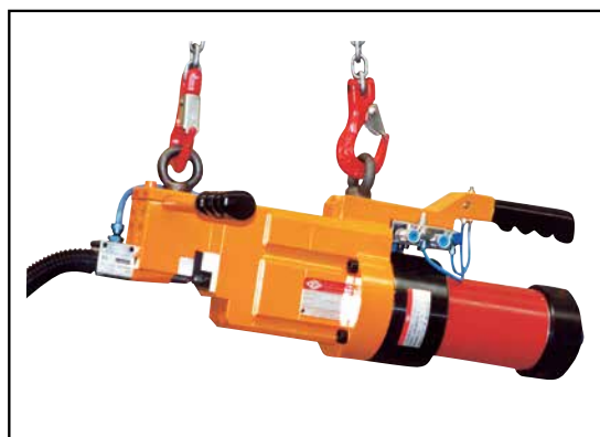
Mobile punching unit for holes Ø 6,2 in crossbeams
